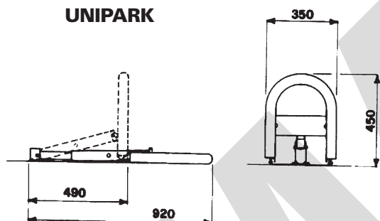
UNIPARK
