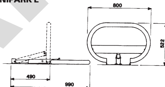
UNIPARK L
