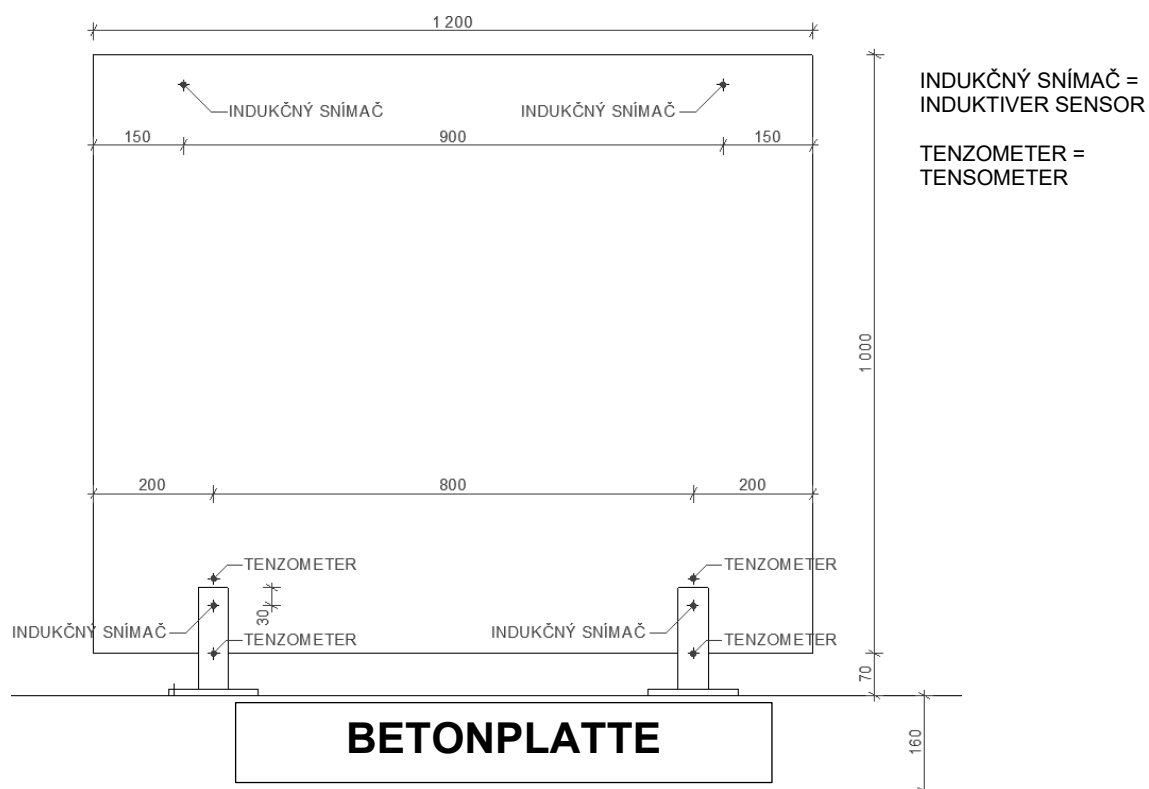
Diagram of the 2x SPIGOT assembly
