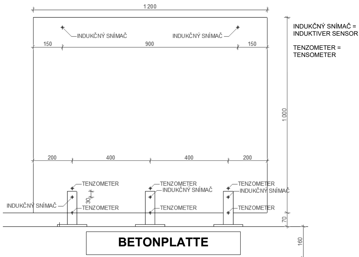
Diagram of the 3x SPIGOT assembly
