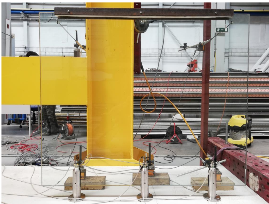
3x SPIGOT assembly
